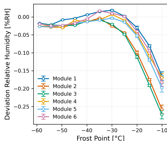
Figure 2: Deviation of the relative humidity signal ( y -axis) of HYT 939p K5 humidity modules as a function of the frost point temperature ( x -axis), including the calculated standard deviation (error bars).
