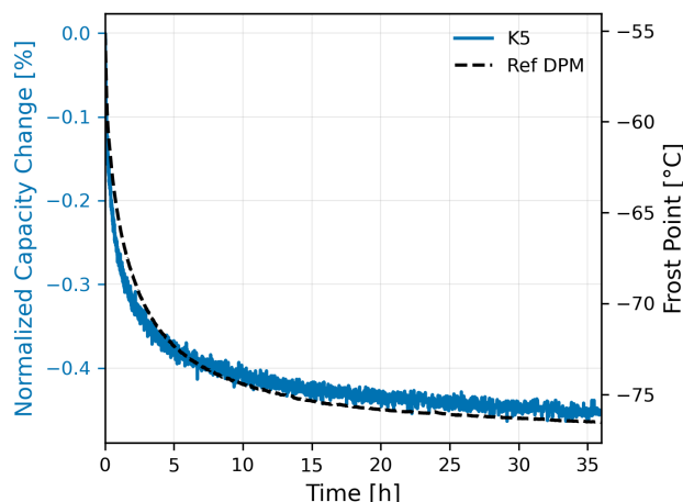
Figure 1: Drying curve of a K5 sensor over time down to a frost point below -75\text{ }^{\circ}\text{C} ( y_1 -axis). The sensor's response aligns with the drying curve measured by the humidity reference (dew point mirror), which indicates the frost point ( y_2 -axis).
