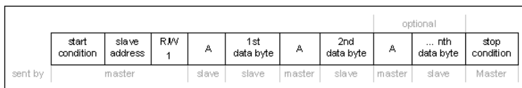
Typical read operation timing sequence
